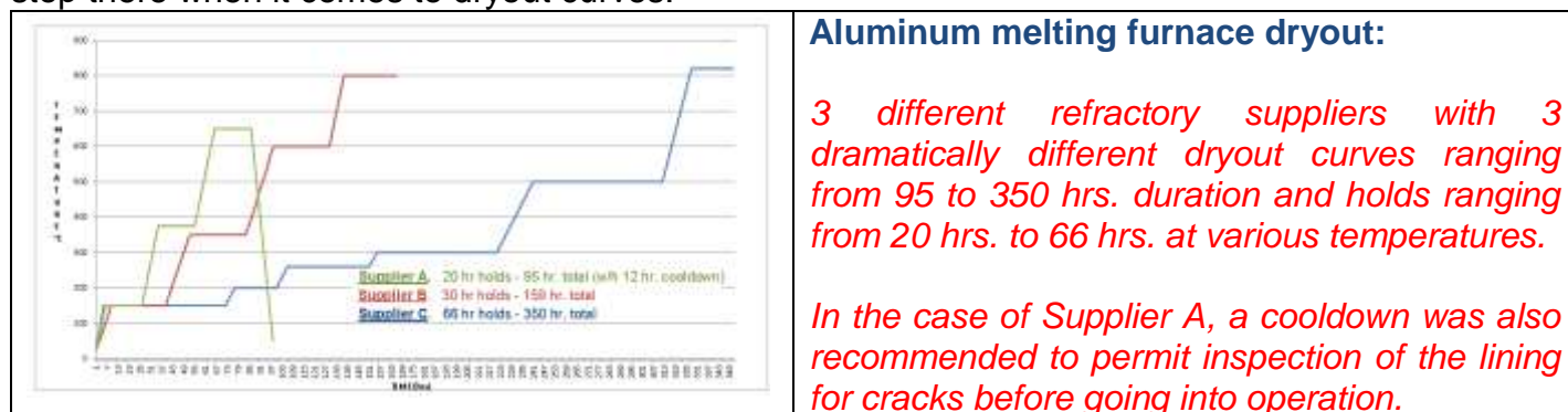
Figure 15: Variation in dryout curves - Aluminum melter
