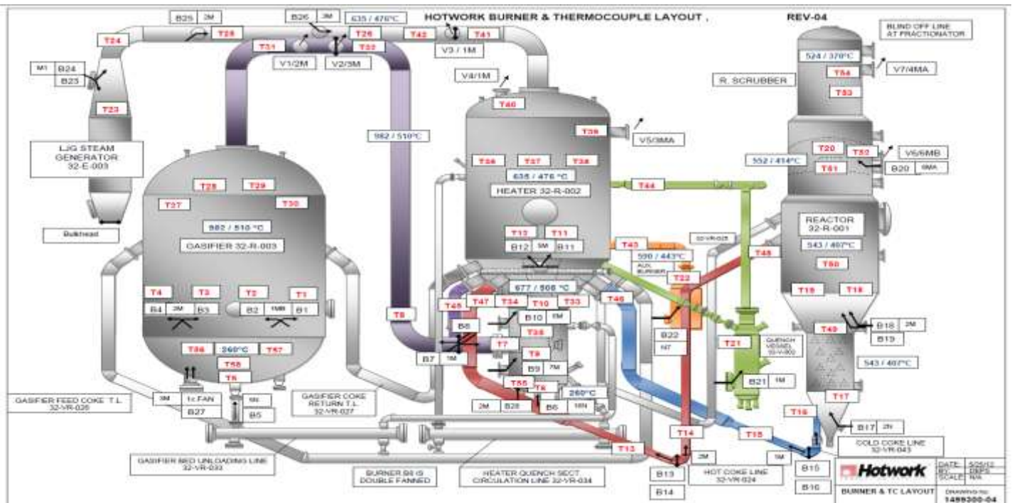
Figure 21: Oil Refinery (26 burners - 58 thermocouples).
