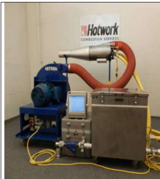
Figure 1: Portable combustion set
